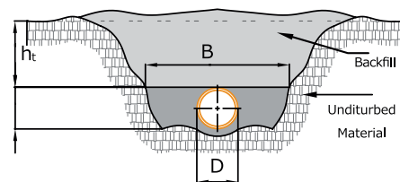
Wide Trench
