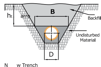
Narrow Trench
